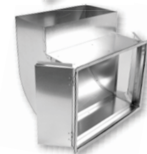
SLA-5U Cold Air Boot w/ adhesive for 5" Filter – Universal Side Load
